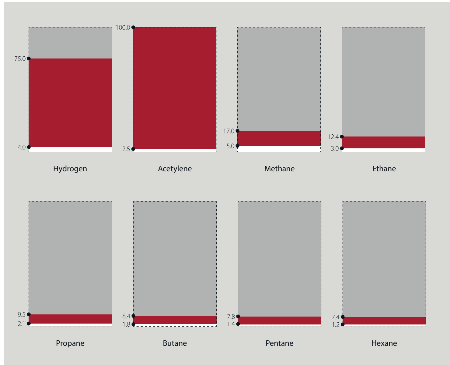
Figure 4: Flammable ranges for eight key gases.
